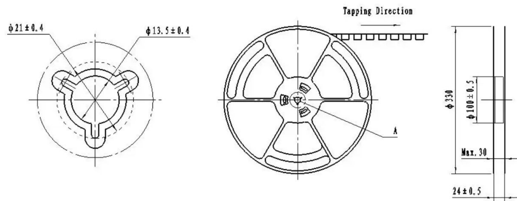
Dimension of Plastic Reel
