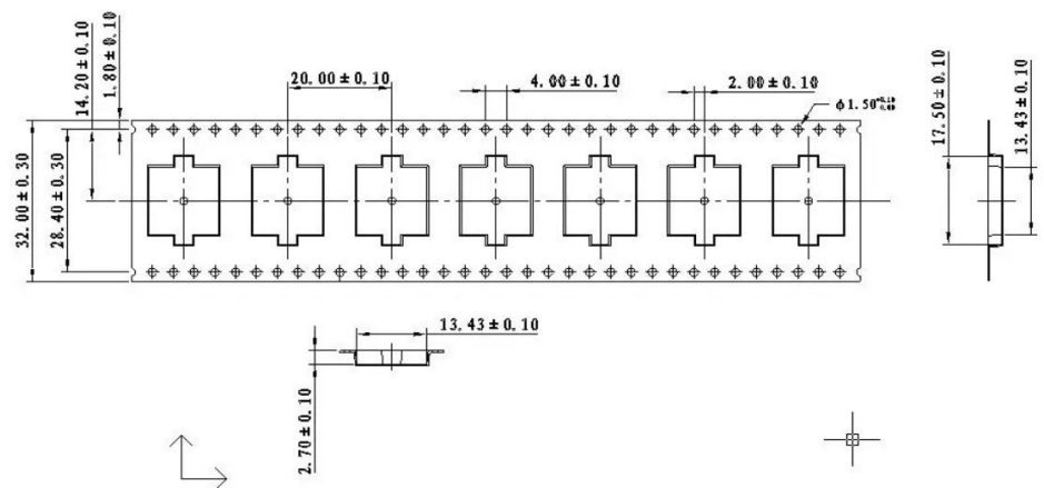
Dimension of Carrier Tape
