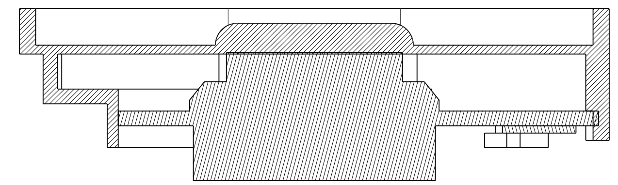
Section B-B
